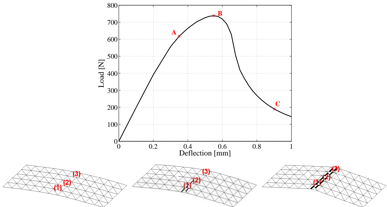
Fig. 15. Structural response of the masonry panel with deformed configuration at different stages of the cracking process.
