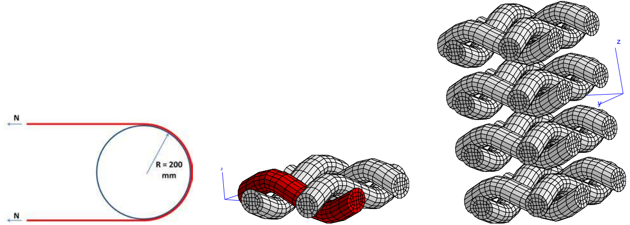
Fig. 3. Plain weave reinforced composites unit cells investigated: (left) loading scheme, (center) single layer RVE (the highlighted warp yarn will be the depicted in the stress maps), (right) RVE for stacking of four plain weave plies.
