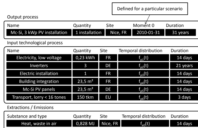
Figure 2: Unit process description of a multi-crystalline (mc-Si) 3 kW p PV installation and its technological inputs and emission.
