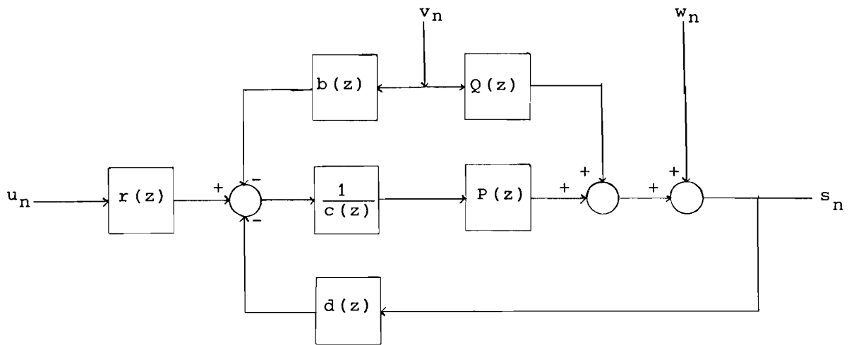
FIGURE 3 - Closed-loop system
