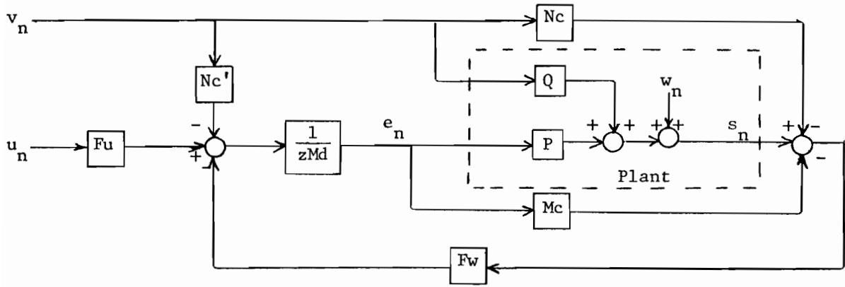
Figure 6. SISO AMAC Representation
