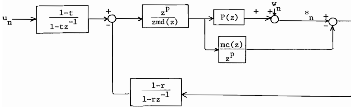
Figure 9. AMAC Representation for Study
