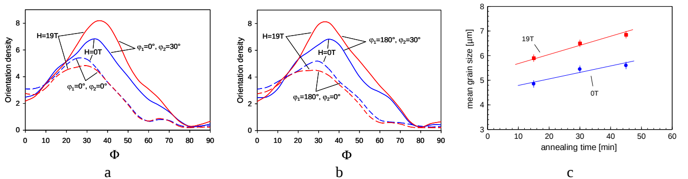
Fig. 2. Orientation density along the fibers a) \varphi_1=0^\circ , \varphi_2=0^\circ as well as \varphi_1=0^\circ , \varphi_2=30^\circ , and b) \varphi_1=180^\circ , \varphi_2=0^\circ as well as \varphi_1=180^\circ , \varphi_2=30^\circ after annealing at 550°C for 45 min at zero field and at 19 T, respectively; c) mean grain size vs. annealing time for specimens annealed at 550°C without field and in a field of 19 T.
