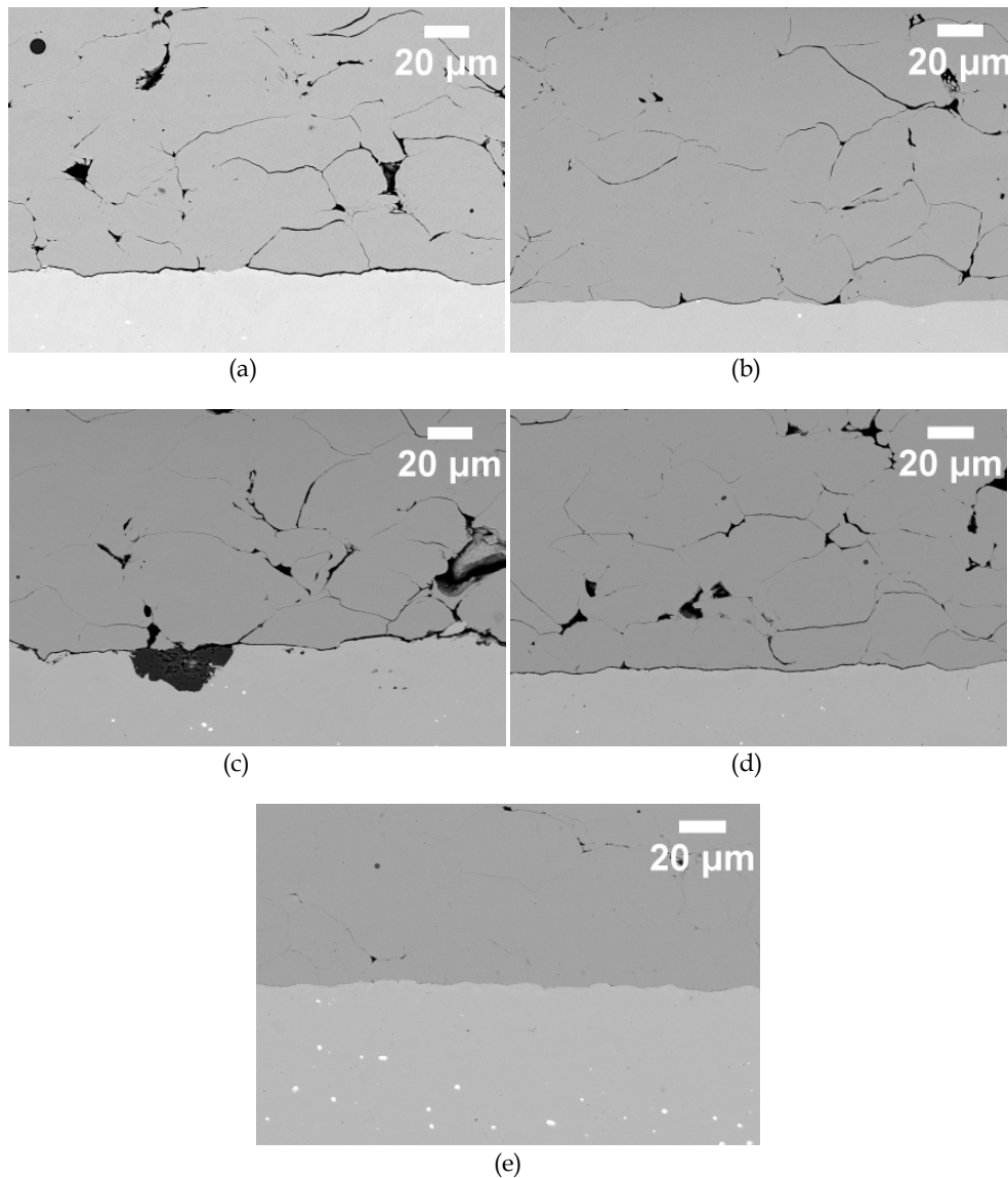
Fig. 25. SEM of cross-sections of cold-sprayed Al coatings formed onto (a) as-received substrate, (b) mirror-polished substrates, (c) grit-blasted substrate (d) laser irradiated substrate ( 1.0 \text{ J}\cdot\text{cm}^{-2} , 18.75 Hz) (e) laser irradiated substrate ( 2.2 \text{ J}\cdot\text{cm}^{-2} , 37.5 Hz).
