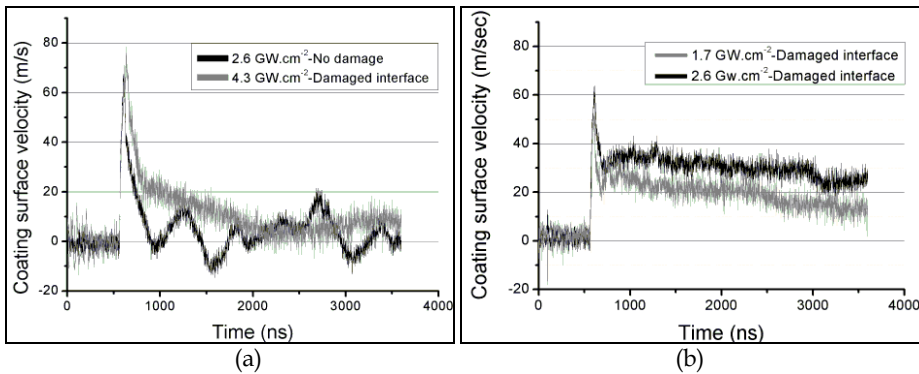
Fig. 20. Velocity profiles of cold-sprayed Al surface on (a) as-received AISI 1070 substrate (b) laser pre-treated ( 2.2 \text{ J.cm}^{-2} ) substrate AISI 1070
