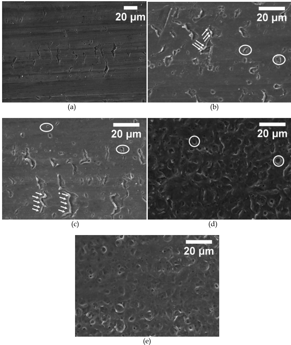
Fig. 12. SEM top view of AISI-2017 substrate surfaces: (a) un-treated and Nd-YAG laser treated (b) 1.0 J.cm -2 , 37.5 Hz., (c) 1.0 J.cm -2 , 150 Hz., (d) 2.2 J.cm -2 , 37.5 Hz., (e) 2.2 J.cm -2 , 150 Hz.
