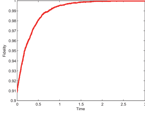
Figure 1: The average fidelity between the Markov processes \rho and \hat{\rho} , over 500 realizations, time t from 0 to T = 3 with discretization time step dt = 10^{-4} .
