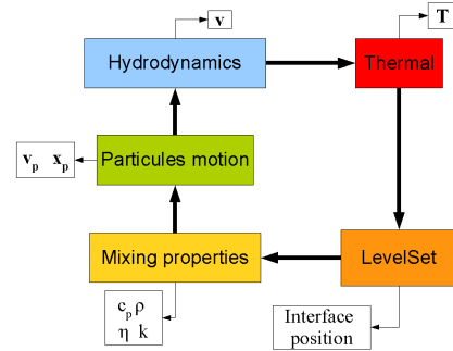
Fig. 3 – Numerical algorithm
