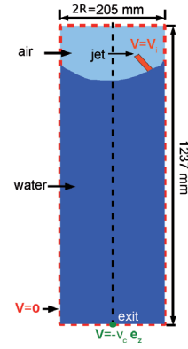
Fig. 5 – Boundary conditions
