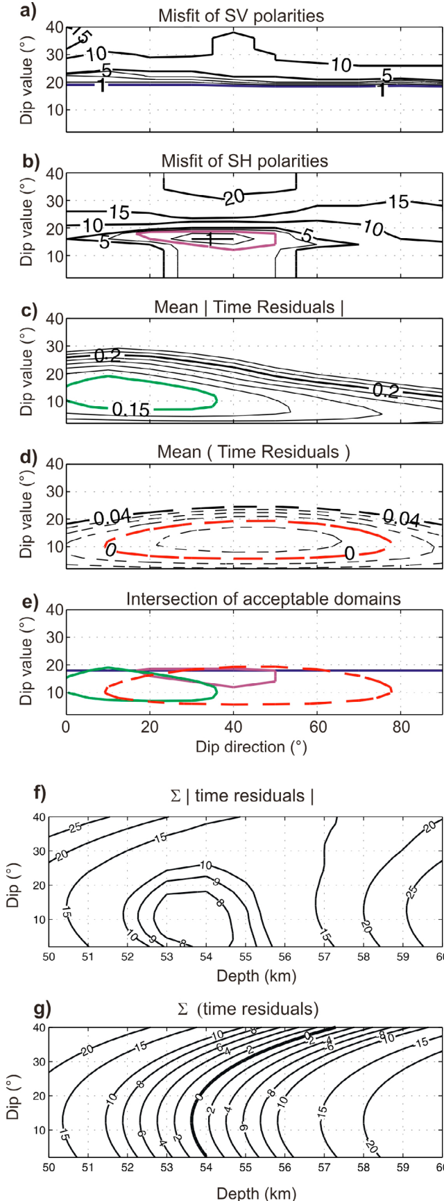
Figure 2. Station VLI. Grid search of model space for depth, dip angle value and dip direction azimuth of the slab top to minimize differences between model synthetics and observations of conversion times and polarities. Horizontal axis is dip direction azimuths from N to N 90°E and vertical axis is dip angle values from 0 to 40°. (a) Number of polarity misfits of 44 data of converted S on the SV, i.e., Q-RF. (b) Number of polarity misfits of 25 data of converted S on the SH, i.e., T-RF. (c and d) Mean of absolute values, respectively of algebraic values in seconds of time residuals, observed-synthetics, computed for a 54 km depth to the top of the slab derived from our analysis in Figure 2e and 2f. (e) The preferred dip azimuth on horizontal axis and dip angle on vertical axis are defined by the intersection of curves enclosing minima of acceptable domains of Figure 2a in blue, Figure 2b in magenta, Figure 2c in green, and their intersection by the dotted red curve of Figure 2c. (f and g) Horizontal axis is slab top depths from 50 to 60 km and vertical axis is dip angles value from 0 to 40° for respectively minimizing the mean of absolute and zeroing the sum of algebraic values in seconds of residuals of observed-synthetic times.
