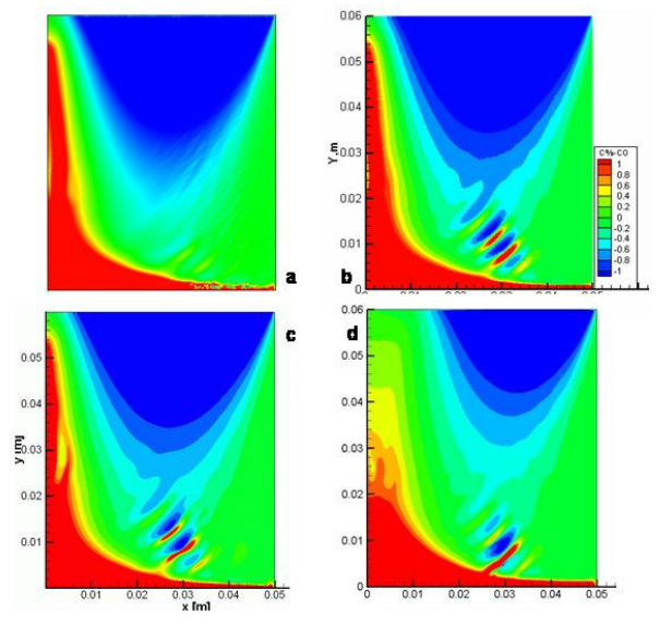
Figure 5: Final maps of segregation ( C - C_0 in wt%Pb) obtained by the four contributors
