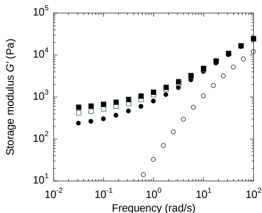
Fig. 1. Variations of storage modulus G' with frequency at 200°C for the matrix (PP/PP-g-MA, \circ ) and for the nanocomposites annealed at 200°C for 20 min ( \bullet ), 130 min ( \square ) and 300 min ( \blacksquare ).
