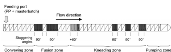
Fig. 1. Screw profile representation
