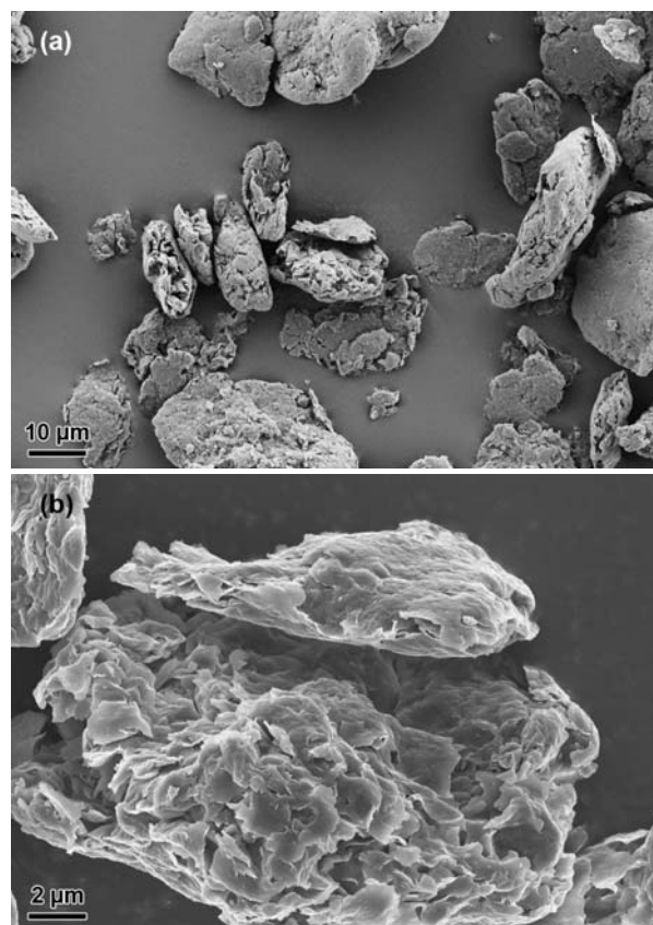
Fig. 2. SEM micrographs of Dellite 67G powder captured with secondary electron detector at different magnifications, (a) \times 1000 , (b) \times 5000
