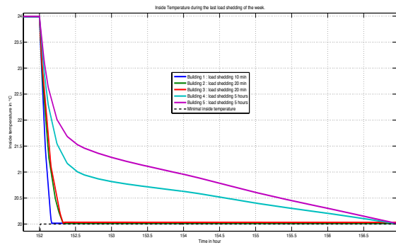
Fig. 4. Comparison of the optimal inside temperature during the load shedding of the last day of the week
