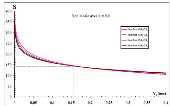
Fig.4. Graphical results method in average non local. We note that the interlaminar tensile strength of interface is relative low compare with interlaminar shear strength. However, this results is correlated
