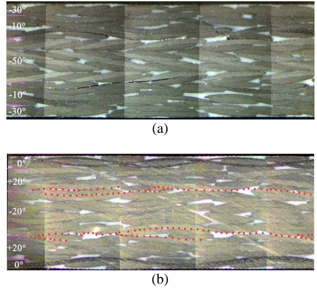
Fig.1. (a) Mixed-mode and (b) open-mode delamination during static loading.
