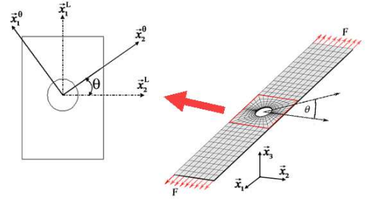
Fig.3. Circular-hole specimen
