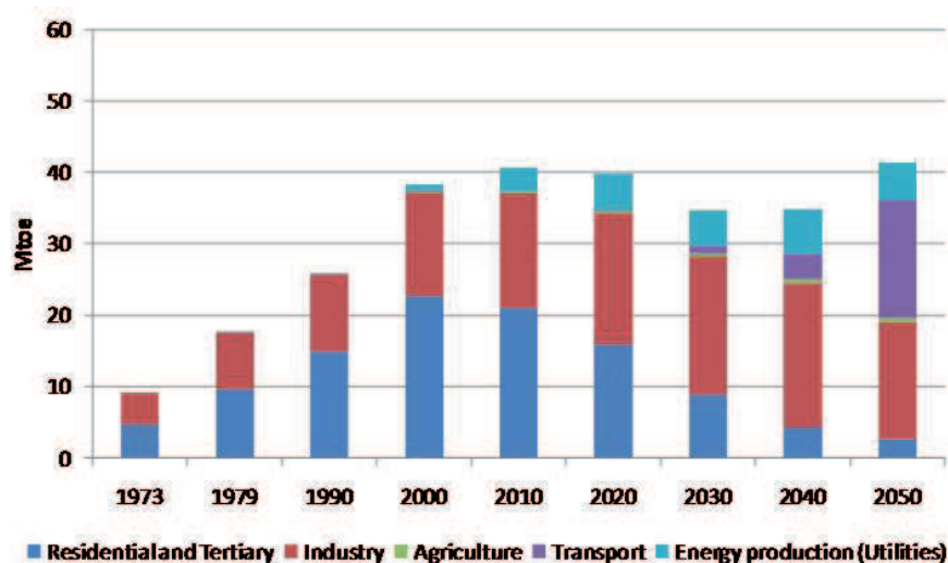
Figure 6. Evolution of natural gas consumption and allocation in the ‘Target’ scenario
