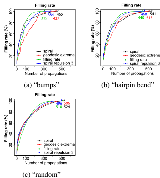
Fig. 9. Comparison of the filling rates, of the array of distances, for the methods: spiral, geodesic extrema, the method based on the filling and the spiral method with a repulsion distance of 3 pixels for the images "bumps", "hairpin bend" and "random".
