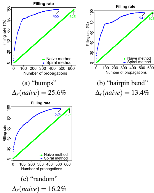
Fig. 4. Comparison of the filling rates \tau of the distances array, between the naive method (in green)
