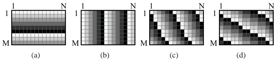
Figure 3: Image corridors (discrete lines) mapping for different SE orientations (a) a horizontal SE, (b) a vertical SE, and (c) and (d) inclined SEs.
