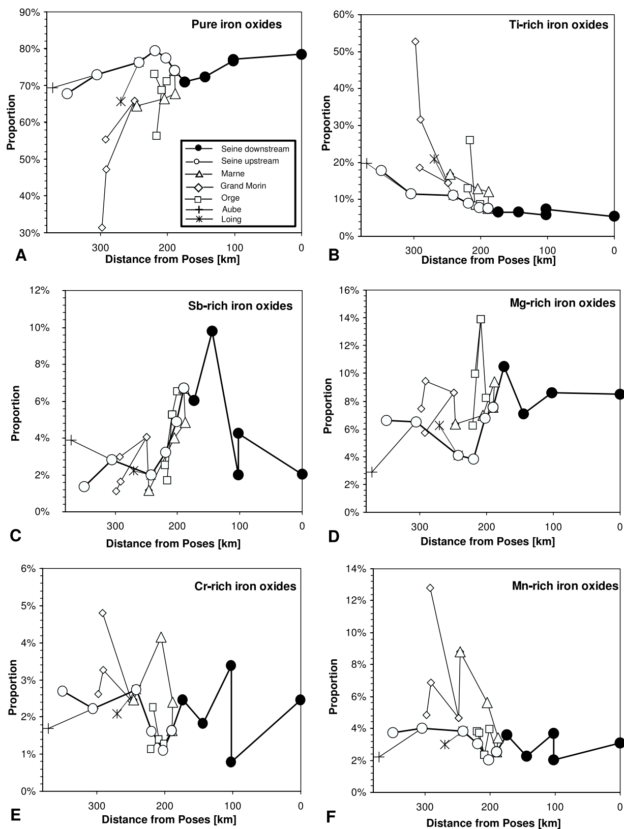
Figure 7. Schematic river-wise presentation of the proportions derived from SEM ACC analysis with respect to the distance from the last sample site Poses: (a) pure iron oxides, particles class 1; (b) Ti-rich iron oxides, particle class 2; (c) Sb-rich iron oxides, particle class 3; (d) Mg-rich iron oxides, particle class 4; (e) Cr-rich iron oxides, particle class 5; and (f) Mn-rich iron oxides, particle class 6.
