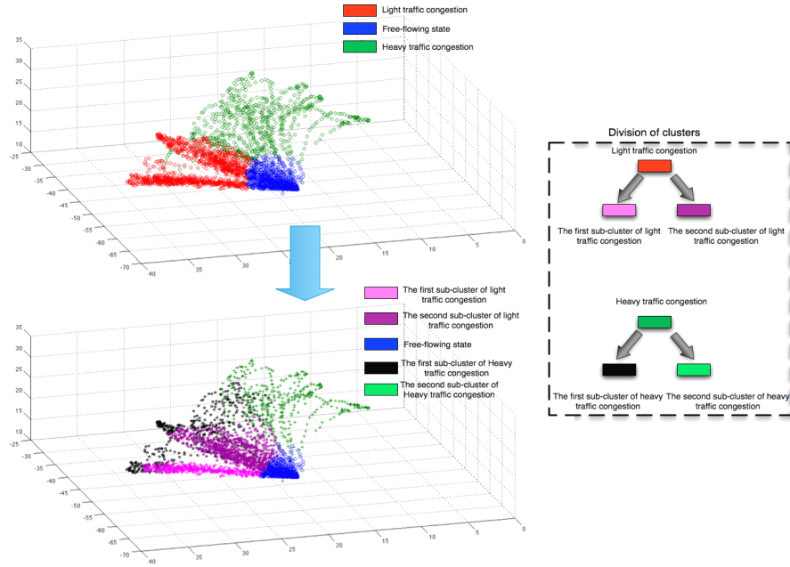
Figure.5 Division of clusters after increasing the number of clusters
