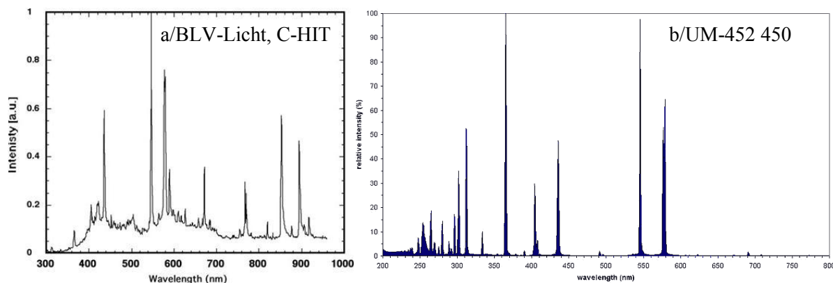
Fig. 1. Irradiation spectrum of the sources used at a) the LMSPC, Strasbourg, France ( ) and b) the Institute of Advanced Energy, Kyoto, Japan (UM-452 450 W)
