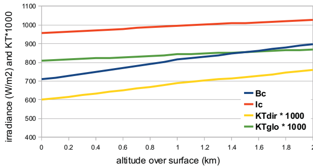
Figure 1. Example of change in irradiance ( B_c for direct and I_c for global) and clearness index (KT) with altitude. KT_{dir} and KT_{glo} are direct and global KT.
