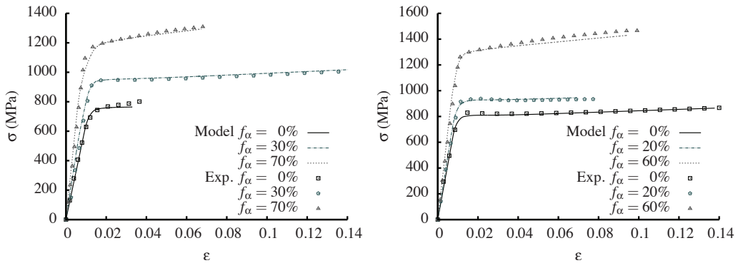
Figure 2: Macroscopic uniaxial tensile tests [pc 1-2] and fitted model predictions for Ti17 microstructures (left) and Ti5553 ones (right)
