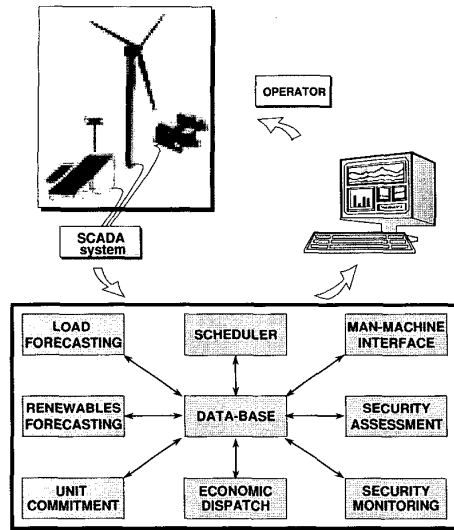
Fig. 1: The CARE system architecture.
