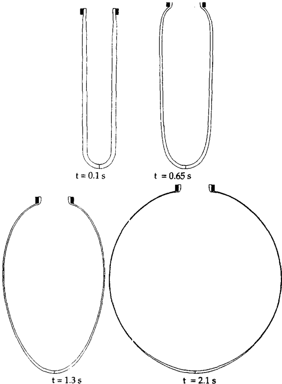
Fig. 14. Intermediate bubble shapes ( T = 105^\circ\text{C} ).
