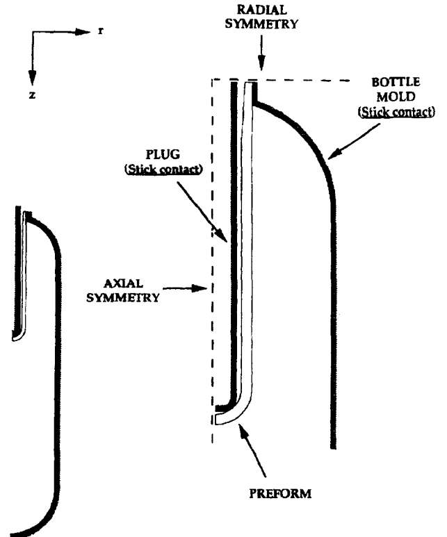
Fig. 11. Boundary conditions.
