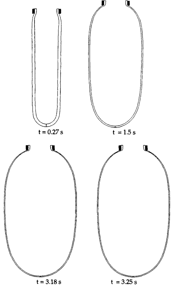
Fig. 15. Intermediate bubble shapes ( T = 105^\circ\text{C} , \bar{E}_0 = 125\% ).
