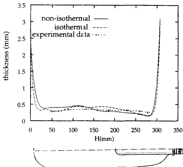
Fig. 19. Thickness distribution at the end of the process.
