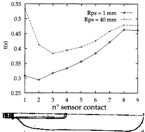
Fig. 6. Contact times versus number of contact sensors.
