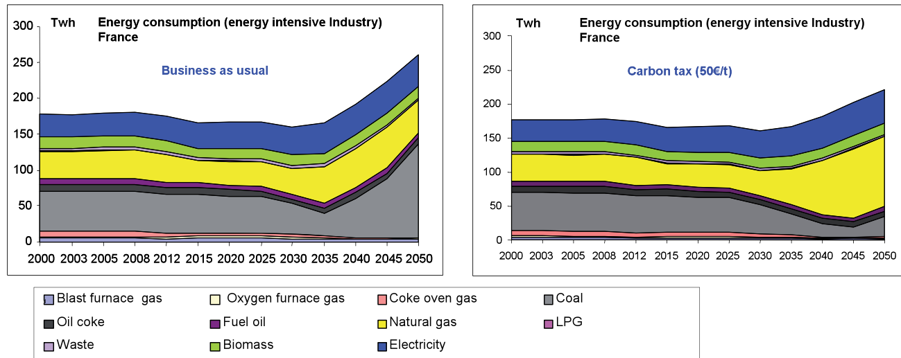
Figure 5: energy consumption, with or without a carbon tax
