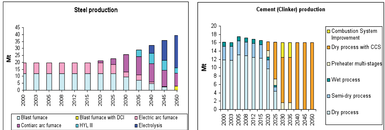
Figure 10: Steel and cement industry response to factor 4 (process change)
