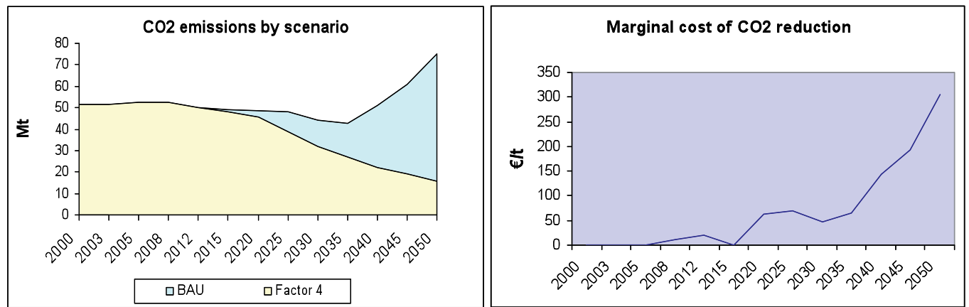
Figure 9: CO 2 emissions and CO 2 marginal reduction cost for large energy consuming industries in the Factor 4 scenario
