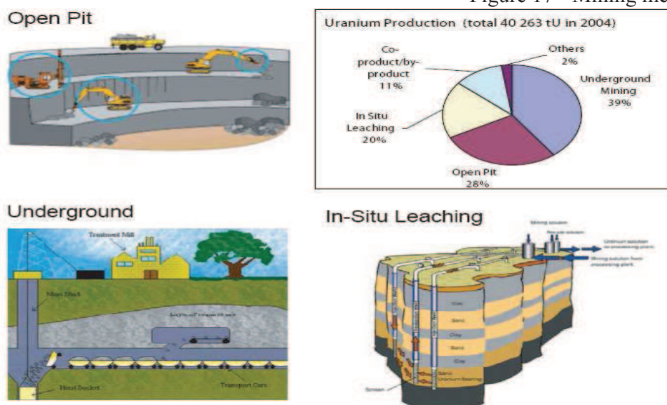
Figure 17 - Mining methods
