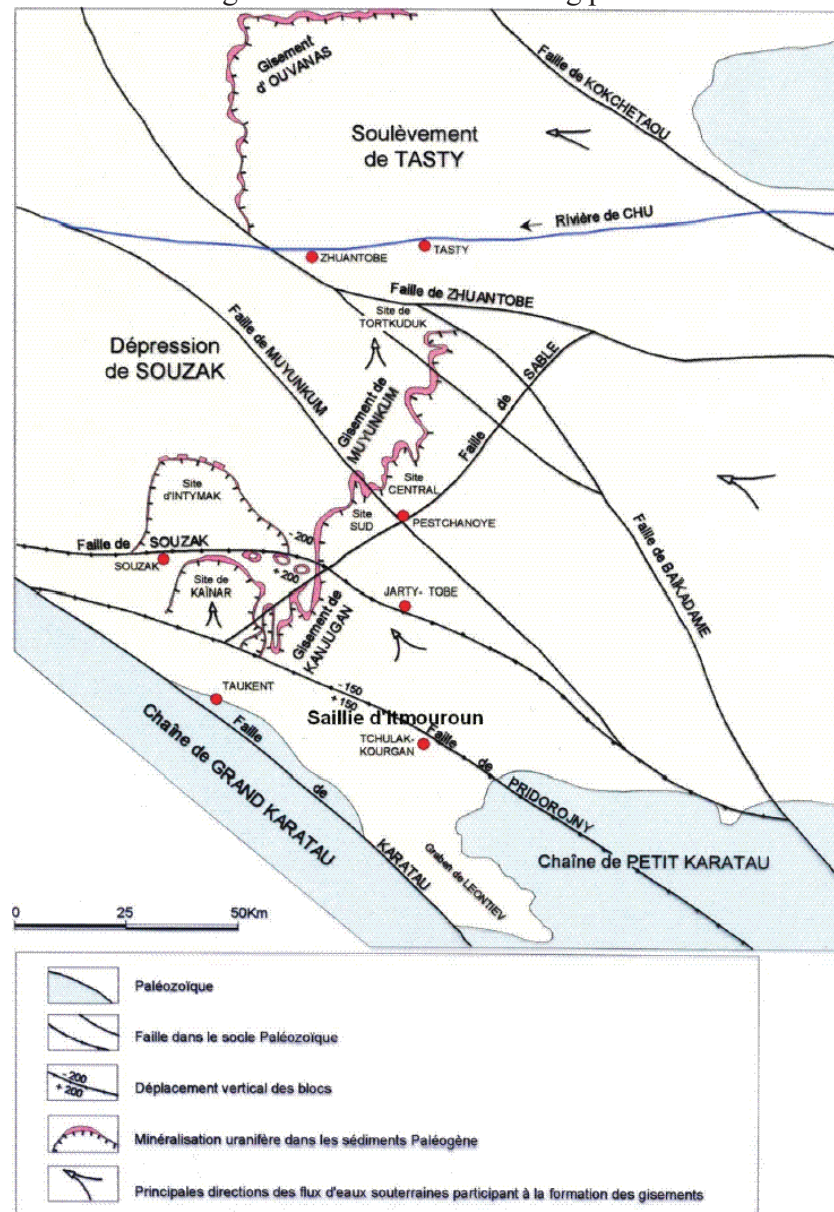
Figure 13 - Structural diagram of the uranium-bearing province of Chu-Saryssu
