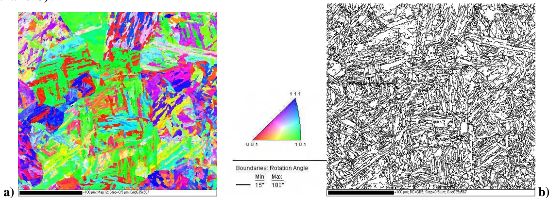
Figure 5: EBSD orientation map a) and boundary map (misorientation >5^\circ ) b) of the base metal.
