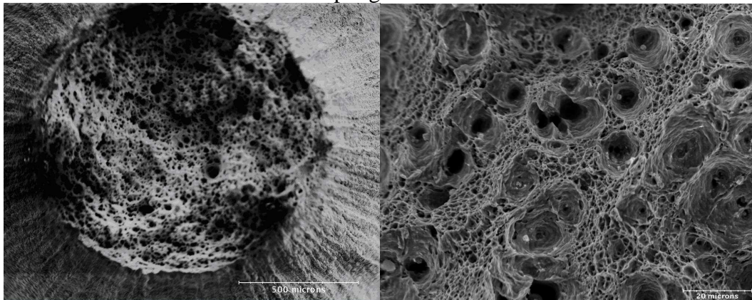
Figure 13: Fracture surface of the crept sample after 2837h (229.6 MPa, 550°C).
