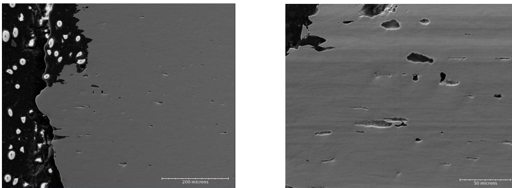
Figure15: SEM observations of damage in the necking area of crept sample (240 MPa, 550°C, cross-section).
