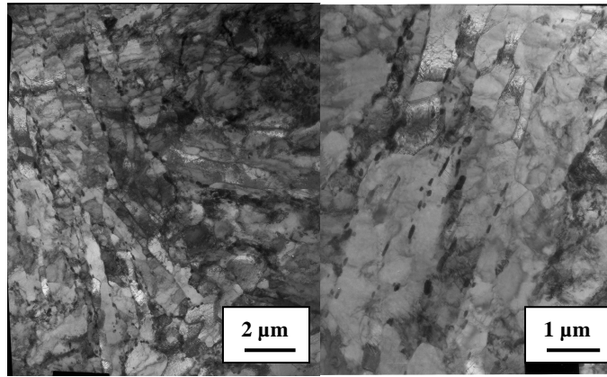
Figure 6: Bright Field TEM observations of the Base metal.
