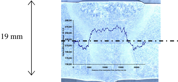
Figure3: Cross-weld microhardness profile combined with observations of the welded joint.
