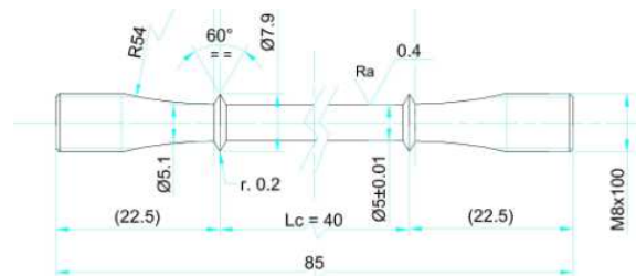
Figure 1: Scheme of creep specimen geometry.
