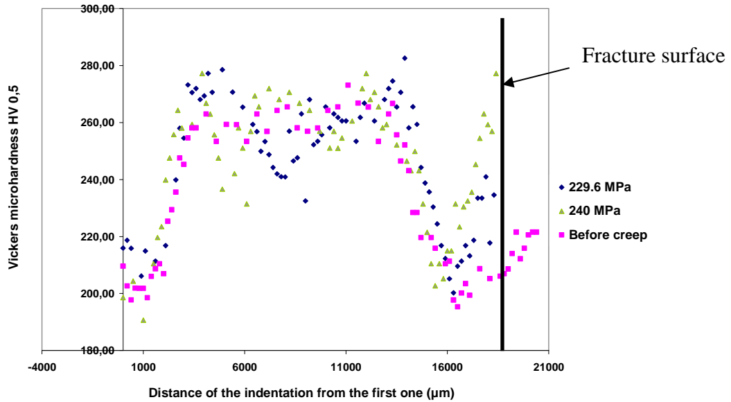
Figure 17: Cross-weld microhardness profiles of two crept specimens
