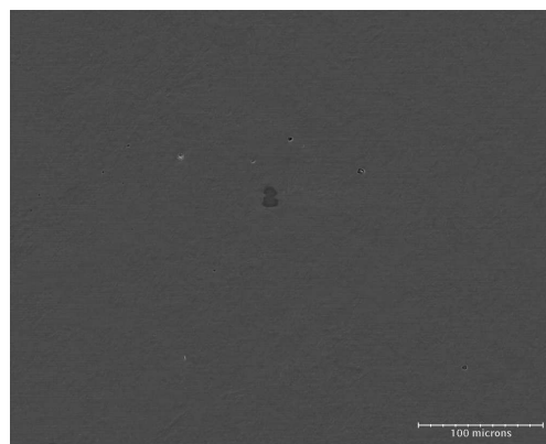
Figure 16: SEM observations of the cross-section of the crept specimen far from the necking area (240 MPa, 550°C).
