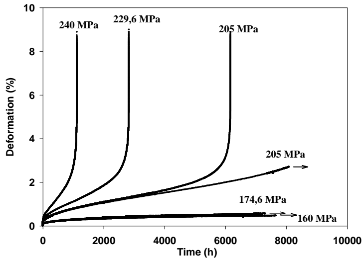
Figure 9: Creep curves at 550°C.
