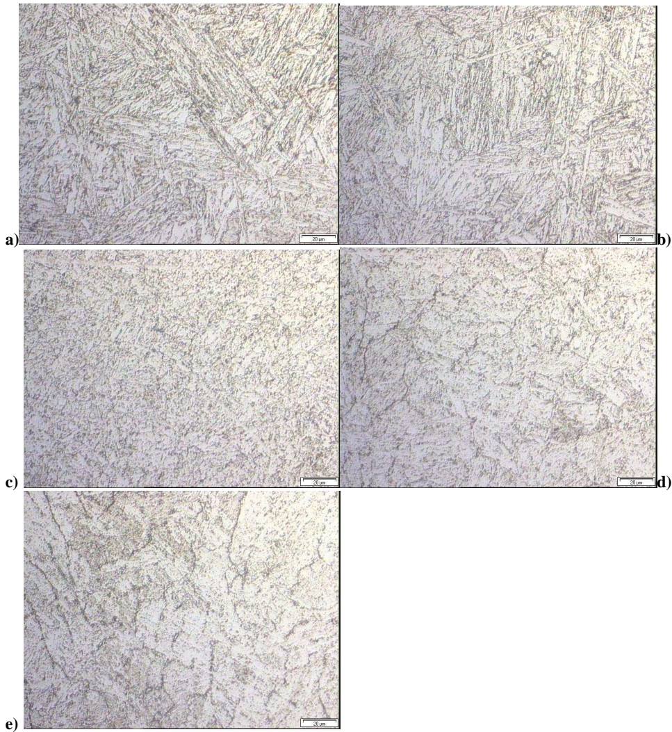
Figure 4: Optical observations of the different areas of the welded joint: a) the base metal, b) the intercritical area, c) the FGHAZ, d) the CGHAZ and e) the weld metal.
