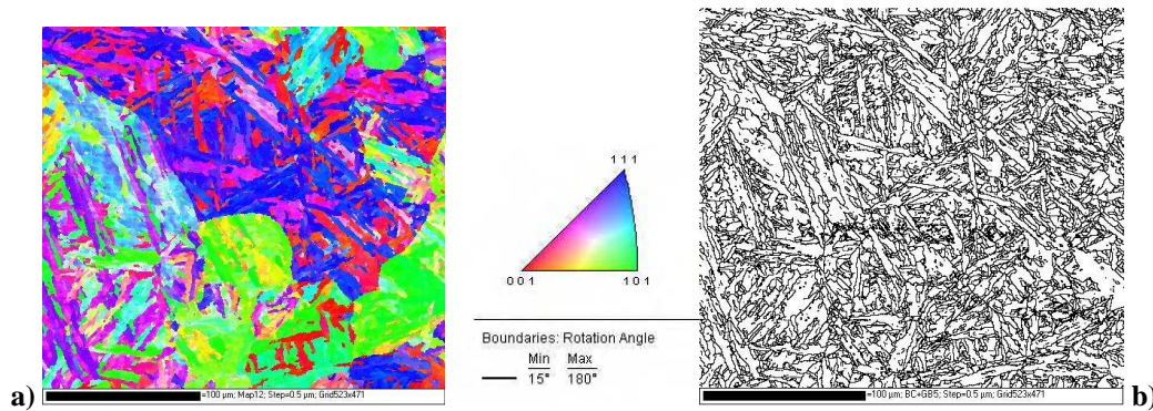
Figure 8: EBSD orientations map a) and boundary map (misorientation >5^\circ ) b) of the softened zone.
