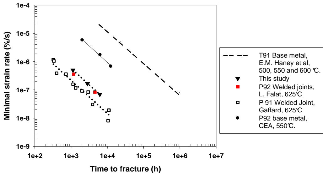
Figure 12: Monkman-Grant curve for crept specimens [8, 9 and 10].
