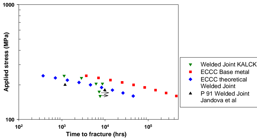
Figure 11: Applied stress versus time to fracture, at 550°C [1, 8].
