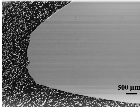
Figure 14: Necking area of a crept sample (240 MPa, 550°C).
