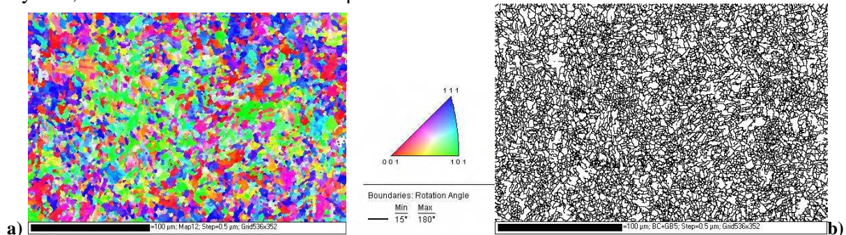
Figure 7: EBSD orientations map a) and boundary map (misorientation >5^\circ ) b) of the fine-grained zone.
