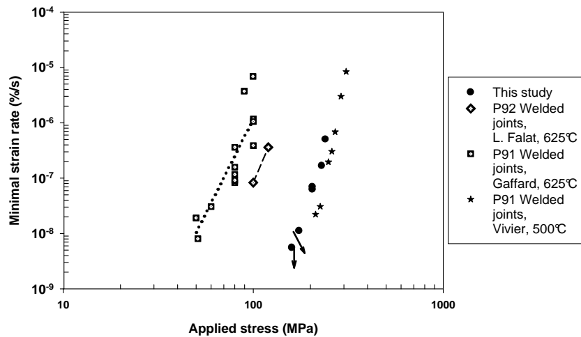
Figure 10: Minimal strain rate versus applied stress for welded joints [3, 6 and 7].
