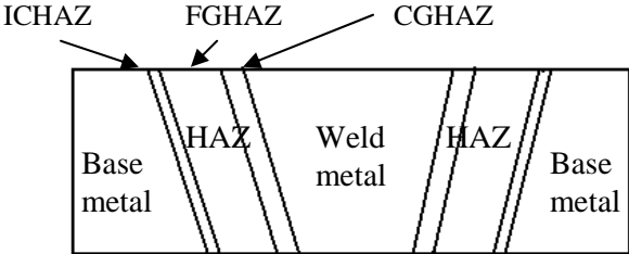
Figure 2: Scheme of the welded joint.
