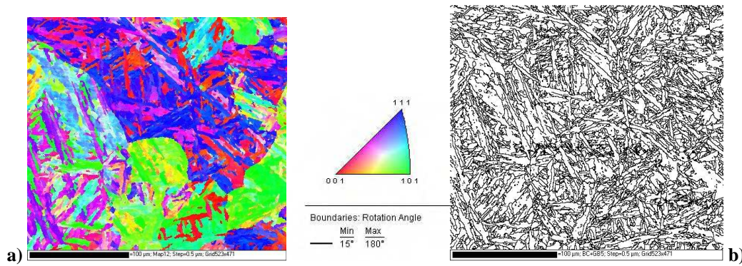
Figure 8: EBSD orientations map a) and boundary map (misorientation >5^\circ ) b) of the softened zone.
