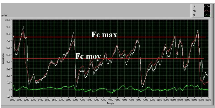
Figure 9 : Experimental PDC forces during rock cutting
