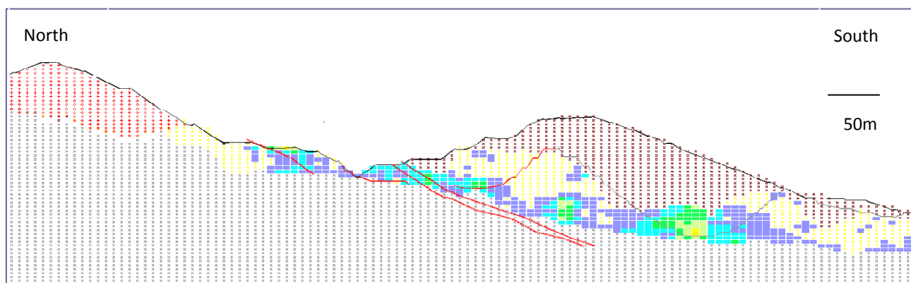
Figure 5 – A North-South section of the current block model
