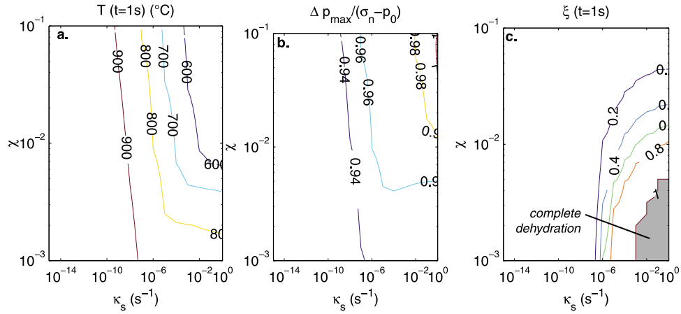
Figure 8. Dependency of (a) T at 1 s of slip, (b) maximum relative pore pressure increase (p_{\max} - p_0)/(\sigma_n - p_0) , and (c) \xi at 1 s of slip on the total amount of water \chi and the kinetics at the onset of dehydration \kappa_s . If the rate constant at equilibrium is very low (from 10^{-15} to 10^{-6} \text{ s}^{-1} ), the effect of dehydration becomes negligible, and the temperature can be much higher than the equilibrium temperature during the reaction. A large constant rate constant promotes small temperature oversteps compared to T_s and a high pore pressure increase.
