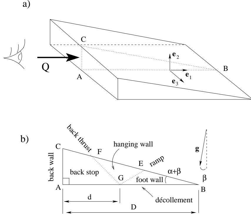
Figure 4: The 3D geometry of the accretionary wedge a) and the central cross-section considered for the 2D analysis, b).
