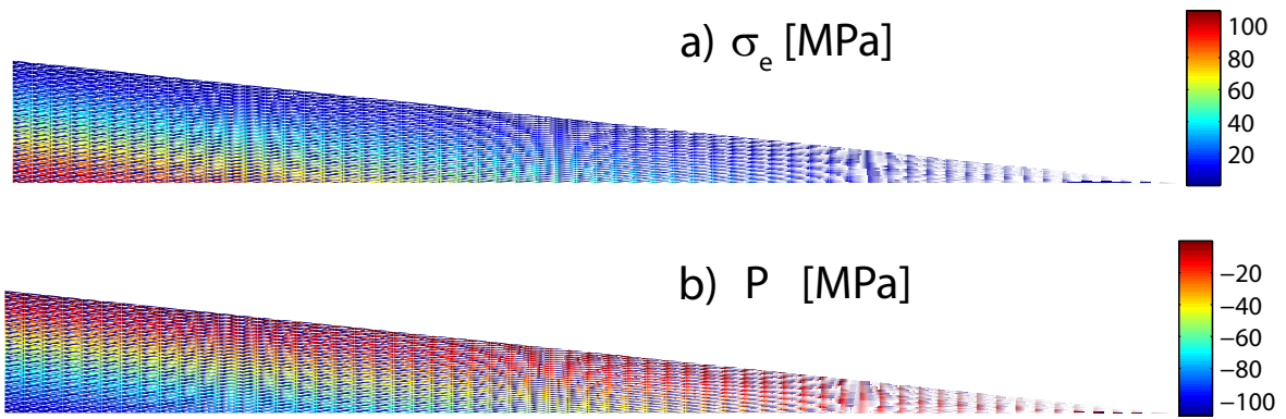
Figure 12: The two stress invariants, the equivalent shear \sigma_e and the in-plane mean stress P in a) and b), respectively, for a back wall friction \phi_{BW} = 5.7^\circ
