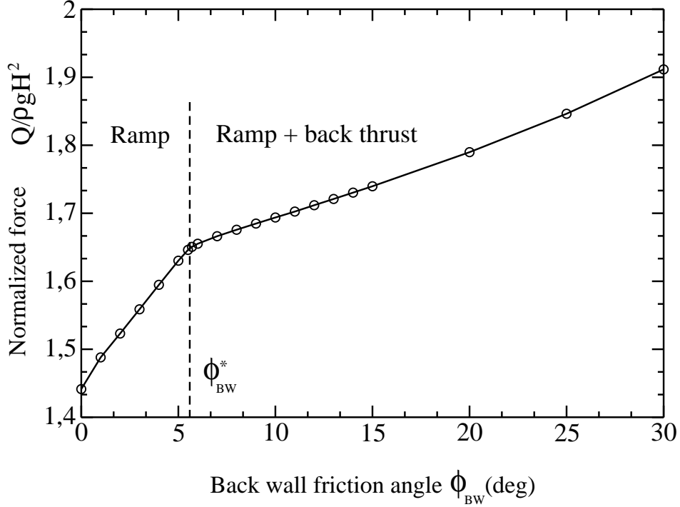
Figure 10: The normalized upper bound to the tectonic force as a function to the friction angles on the back wall.
