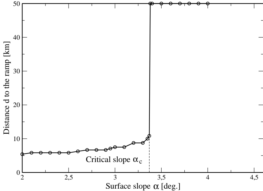
Figure 9: The position of the root of the ramp and back thrust on the décollement as a function of the topographic slope. The dashed line marks the analytical solution of Dahlen (1984). The back-wall friction angle is set to \phi_{BW} = 30^\circ .
