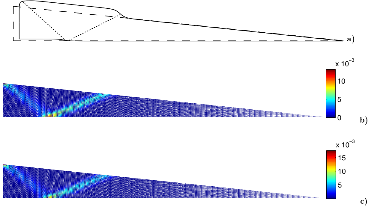
Figure 6: Sub-critical slope conditions: \alpha = 3^\circ < \alpha_c . The deformed boundary of the mesh based on the nodal velocities at the six nodes of each triangle, superposed to the original mesh in dashed lines, a). The dotted segments mark the core of the zone of localized virtual deformation and could be interpreted as the back thrust and the ramp. Iso-contours of the virtual volumetric \hat{\theta} and the virtual equivalent shear strain \hat{\gamma} are presented in b) and c), respectively.
