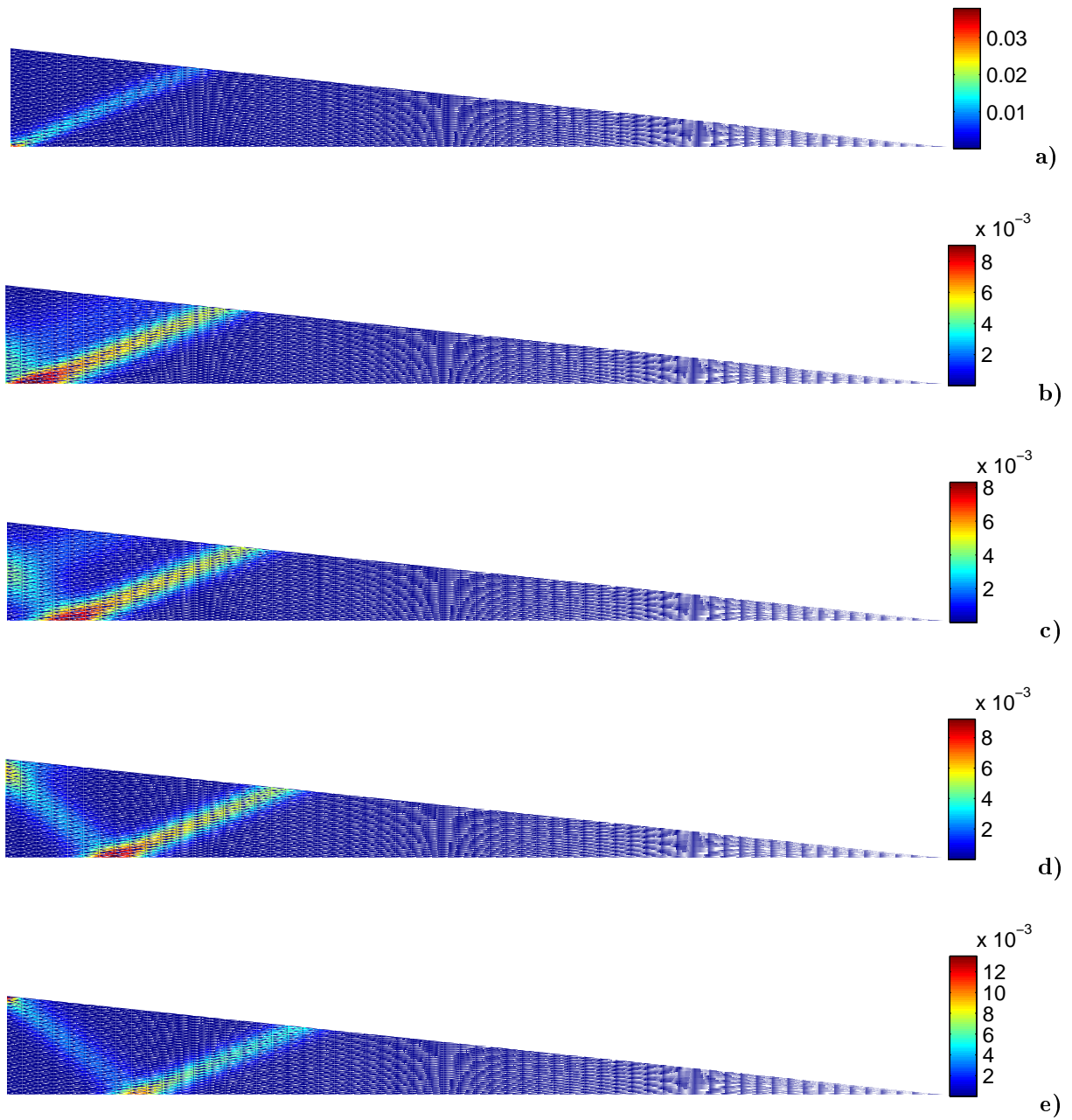
Figure 11: The failure mode for sub-critical topographic slope conditions ( \alpha = 3^\circ < \alpha_c ) for five values of the back wall friction \phi_{BW} set to 3^\circ , 5.5^\circ , 5.7^\circ , 7^\circ and 15^\circ , in a) to e), respectively. Iso-contours of the virtual equivalent shear strain \hat{\gamma} .
