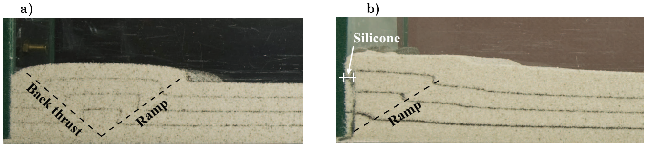
Figure 14: Two pictures of the laboratory experiments from the side showing a ramp and back-thrust for failure mode a) and a ramp only in b) in the absence and the presence of a layer of silicone along the back wall, respectively.
