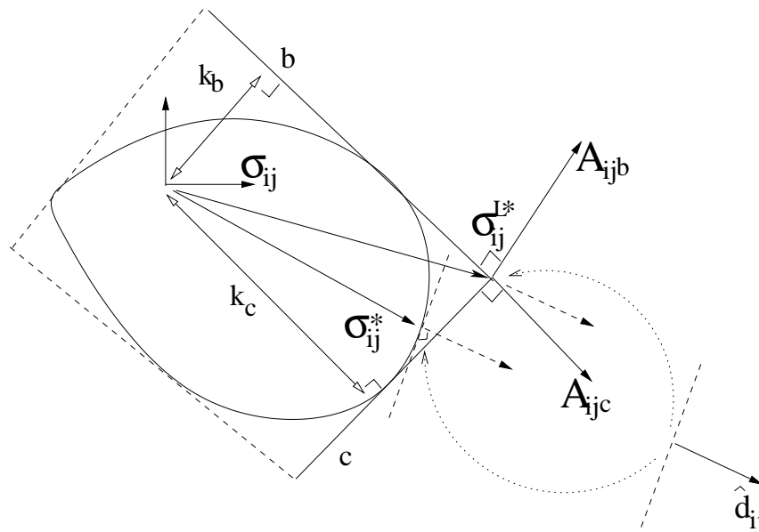
Figure 1: The graphical method to construct the support function for a convex strength domain. The linearized strength domain bounds the support function externally and is represented by four hyper-planes (two dashed and two solid lines).
