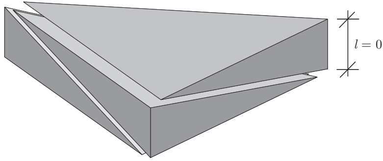
Figure 16: Discontinuity patch consisting of three zero-thickness tetrahedra for constructing a discontinuity of known geometry and zero thickness in 3D.
