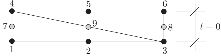
Figure 3: Kinematically admissible velocity discontinuity comprised of two quadratic elements of thickness l set to zero.
