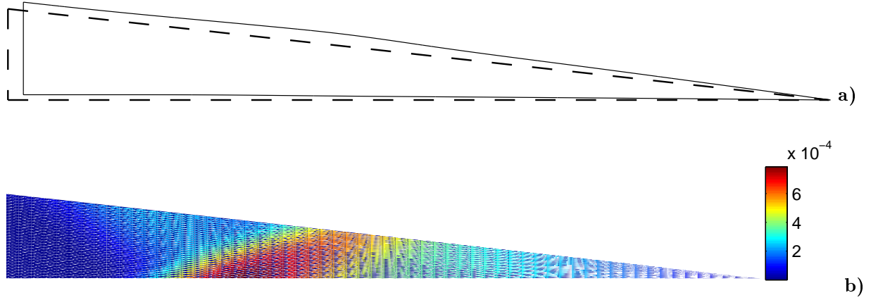
Figure 7: Critical slope conditions: \alpha = \alpha_c . The boundary of the deformed mesh superposed to the original mesh, dashed lines, a) and the iso-contours of equivalent-shear virtual-strain \hat{\gamma} in b). The whole décollement is activated and the deformation is rather diffuse.
