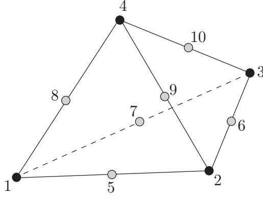
Figure 15: Quadratic tetrahedron element for 3D upper bound analysis.
