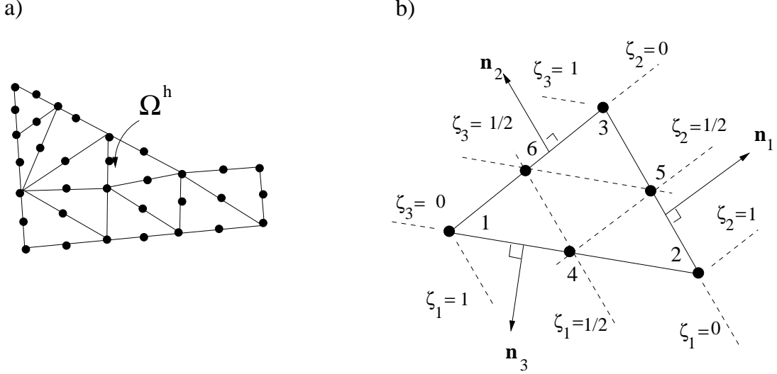
Figure 2: Discretization of the domain \Omega by six-noded triangles, a). The six-noded triangle local node numbering and the definition of the area-coordinates, b)
