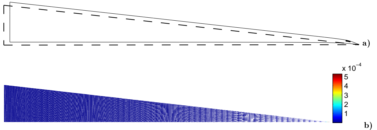
Figure 8: Super-critical slope conditions: \alpha = 3.5 > \alpha_c . The boundary of the deformed mesh superposed to the original mesh, dashed lines, a) and the iso-contours of equivalent-shear virtual-strain \hat{\gamma} in b).
