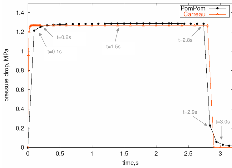
Fig. 4 Pressure drop throughout time for the contraction/expansion test.
