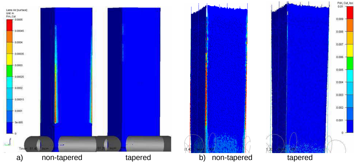
Figure 6. a) Influence of mould tapering on air gap [m] formation. b) Yamanaka et al. [18] criterion projected onto the solidus surface
