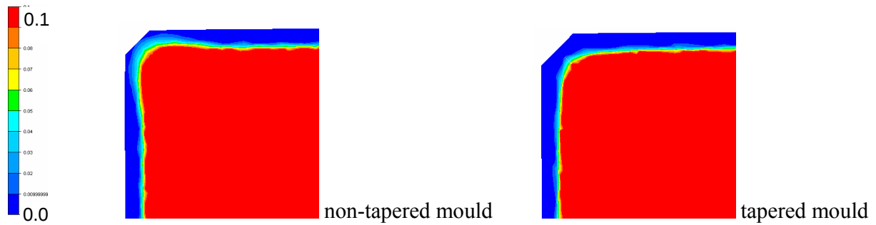
Figure 7. Liquid fraction [0;0.1] showing undersolidification at corner
