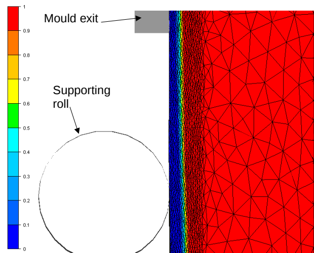
Figure 8. Refined mesh used in solid shell to compute the hot tearing criteria (liquid fraction represented on the picture)
