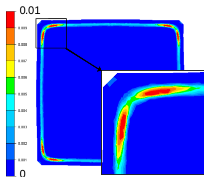
Figure 9. Yamanaka et al. [18] criterion cumulated in the primary and in the secondary cooling
