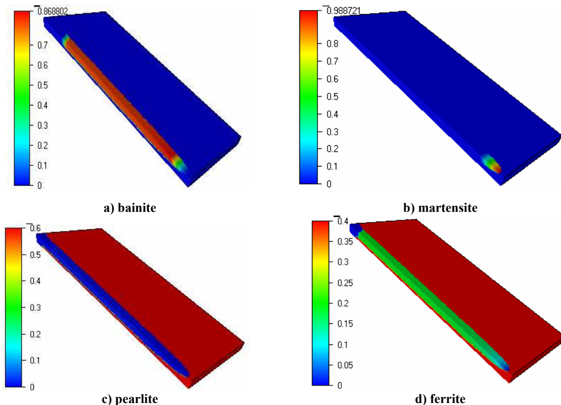
Figure 8. Calculated volume fractions of the different phases at the end of welding.
