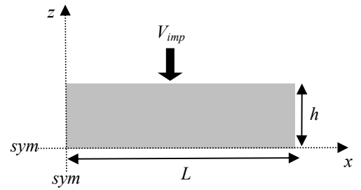
Figure 1. Two-phase simple compression test geometry.
