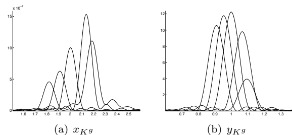
Fig. 5. simulations: Fourier transform of the signals x(t) and y(t) in the frame K^g for different z : z = 0, 0.25, 0.5, 0.75, 0.1 ; (a): oscillation frequencies of x_{Kg} ; (b): oscillation frequencies of y_{Kg} ;
