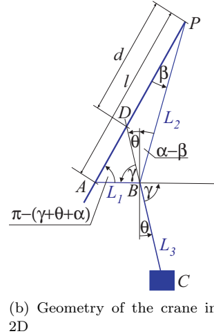
Fig. 3. Geometry of the crane
