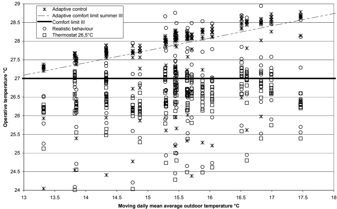
Figure 8 Operative temperatures for three local control strategies in July
