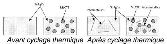
Fig. 1: SnAgCu Matrix reinforced by Mo or SiC (*MLCTE: Material with low coefficient of thermal expansion)
