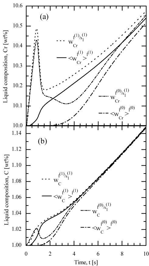
Fig. 5. Time evolutions of the average composition for the interdendritic liquid, \langle w_i^{(1)/s_1^{(1)}} \rangle^{(1)} , and the extradendritic liquid, \langle w_i^{(0)/s_1^{(1)}} \rangle^{(0)} , and the interfacial composition for the extradendritic liquid at the interface with the dendrite tip, w_i^{(0)/s_1^{(1)}} , and the interdendritic liquid at the interface with the primary dendritic solid phase, w_i^{(1)/s_1^{(1)}} , for (a) i=Cr and (b) i=C .
