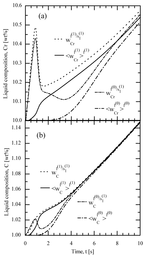
Fig. 5. Time evolutions of the average composition for the interdendritic liquid, \langle w_i^{(1)} \rangle , and the extradendritic liquid, \langle w_i^{(0)} \rangle , and the interfacial composition for the extradendritic liquid at the interface with the dendrite tip, w_i^{(0)/s_1^{(1)}} , and the interdendritic liquid at the interface with the primary dendritic solid phase, w_i^{(1)/s_1^{(1)}} , for (a) i=Cr and (b) i=C .
