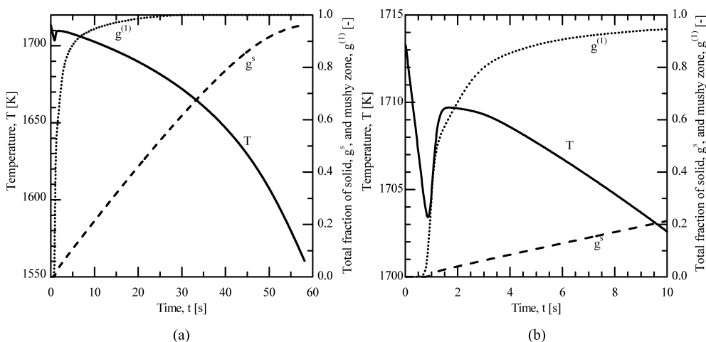
Fig. 2. Time evolutions of the temperature, T (plain line), the total fraction of solid, g^s (dashed line), and the fraction of the primary mushy zone, g^{(1)} (dotted line), upon solidification of a Fe-1wt%C-10wt%Cr alloy.
