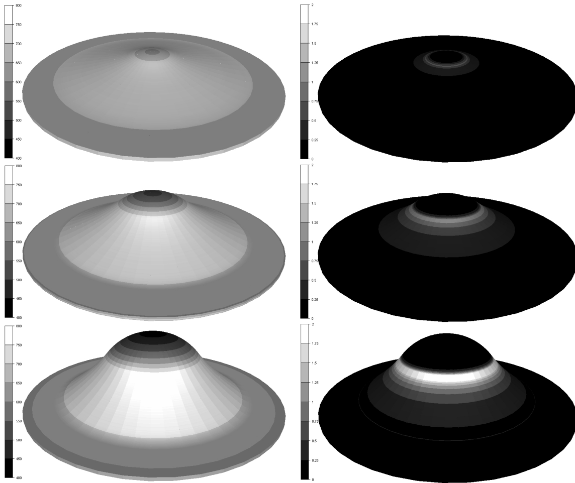
Figure 3. Results of numerical simulation for 10, 20 and 30 mm punch strokes: Evolution of the temperature [°C] (left) and Von Mises equivalent strain rate [1/s] (right)
