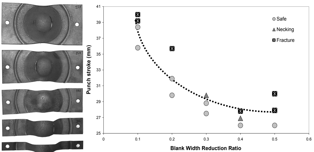
Figure 10. Hot stamped blanks with different width reduction ratios (left) and influence of the blank width on formability (right)
