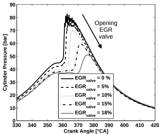
Figure 4. Experimental variation of the EGR valve at fixed operating conditions (5 bar IMEP injection strategy, N_e = 1500\text{rpm} , VGT = 33%). Effect on the cylinder pressure.
