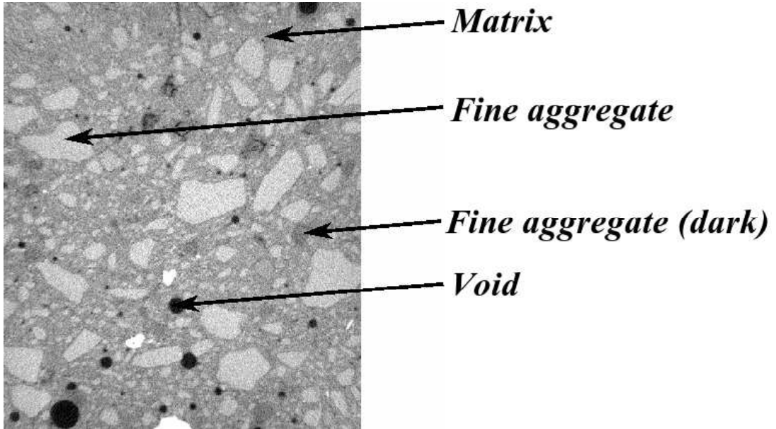
Figure 1: 2D section of a 3D mortar image obtained by microtomography: matrix/cement, light and dark fine aggregates, and voids (strongly dark). The 3D image is of size 2.5 \times 3 \times 2.5 \text{ cm}^3 and of resolution 25 \text{ }\mu\text{m}/\text{voxel} .
