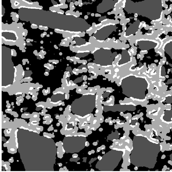
Figure 14: 2D section of the sets used to evaluate the function \rho_a(r) at r = 5 . Aggregate phase (set A_j ) is given in dark gray, A_k \oplus B(r) ( A_k corresponds to regions of high values of the considered stress field component), is given in light gray and their intersection A_j \cap (A_k \oplus B(r)) is given in white.
