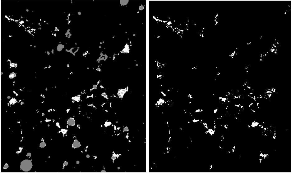
(c) From (b), selection of flat zones (white) by volume thresholding. (d) Removing of pores and zones around (white) by volume thresholding. For pores, using dilation, from (c). comparison, pores are shown in gray.
