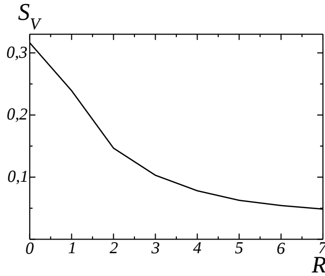
Figure 3: Fine aggregates specific surface area S_V vs. filter size R . This curve is used to determine the optimal filter size, obtained when the specific surface area is close to stabilization.
