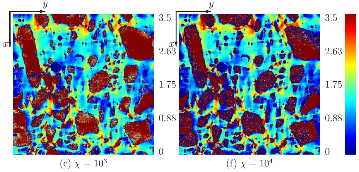
Figure 10: 2D sections of the normalized shear stress component \sigma_{xy}/[E^{(m)}\langle\varepsilon_{xy}\rangle] at varying contrasts \chi = E^{(a)}/E^{(m)} . The field maps are thresholded according to the color-scale as shown on the right. Shear strain loading is applied with \langle\varepsilon_{xy}\rangle = \varepsilon_0 (colors on-line). The 3D image is of size 1.25 \times 1.25 \times 1.25 \text{ cm}^3 and of resolution 25 \text{ }\mu\text{m}/\text{voxel} .
