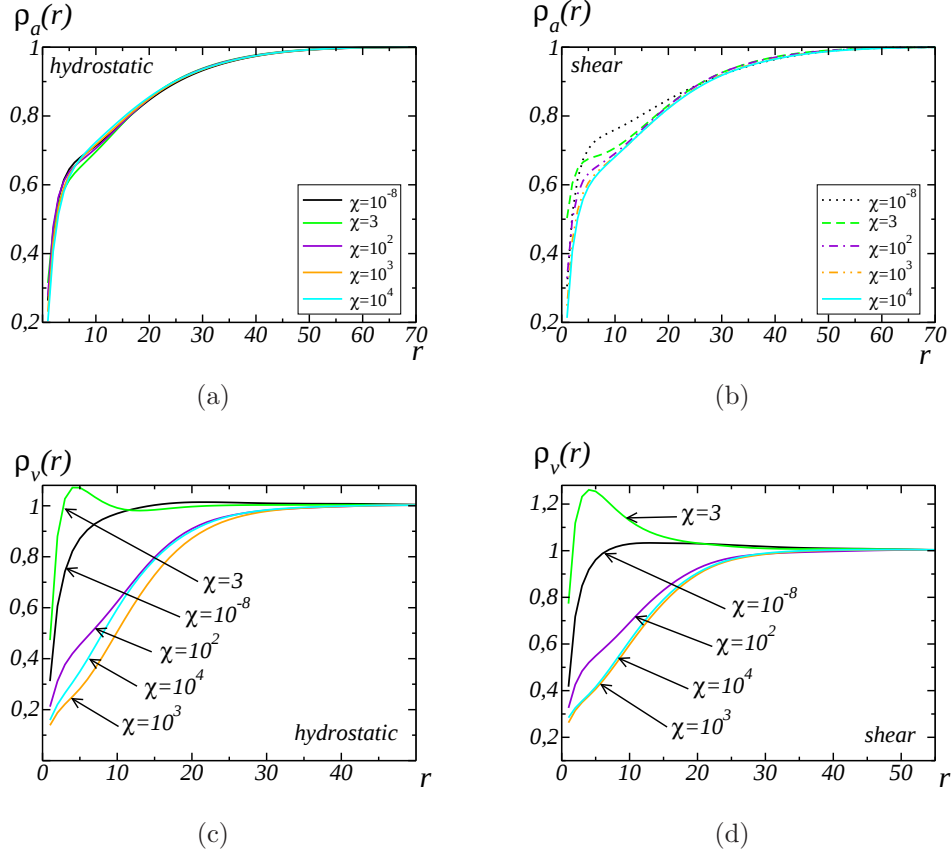
Figure 18: Function \rho_{a,v}(r) used to measure the correlation between one of the material phase (a, b: fine aggregates, c, d: voids) and regions of high-stress. Hydrostatic or shear strain loading is applied (a, c and b, d, resp.). High-stress regions are determined by thresholding the parallel stress component \sigma_m or \sigma_{xy} .
