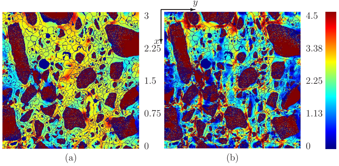
Figure 16: 2D cut at z = cst of the parallel stress component \sigma_m and \sigma_{xy} (maps a and b, resp.) with applied hydrostatic or shear strain loading, resp., with aggregates/matrix contrast \chi = 10^4 . The stress field values correspond to the color scale at right (values outside of the range given at the right of each map are thresholded). The aggregates SKIZ is superimposed on the maps and shown in blue. The 3D image is of size 2.5 \times 3 \times 2.5 \text{ cm}^3 and of resolution 25 \text{ }\mu\text{m}/\text{voxel} .
