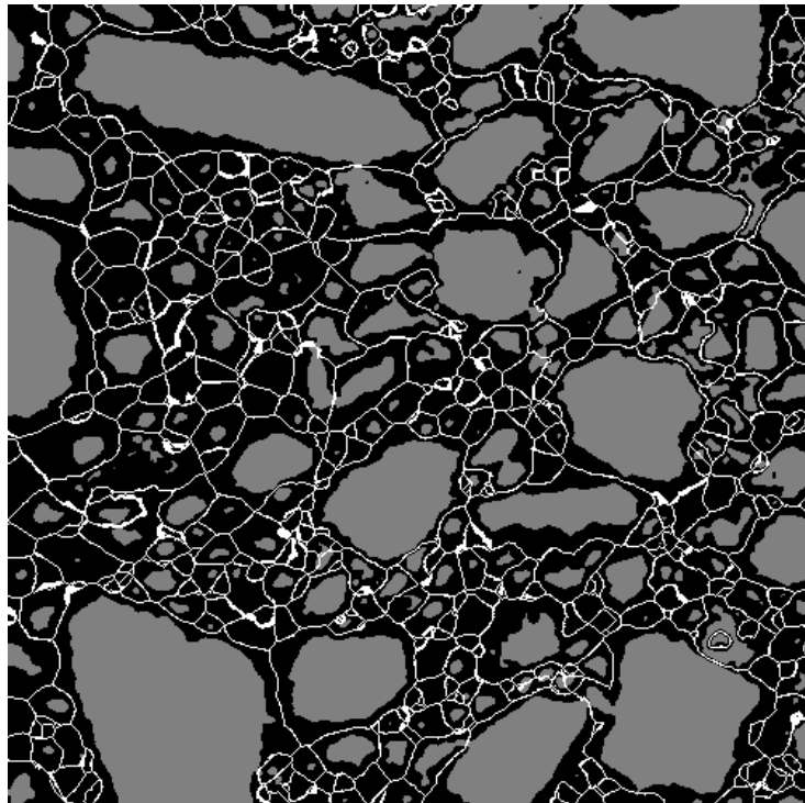
Figure 13: 2D section of the skeleton by influence zone (SKIZ) of the fine aggregates phase. Fines aggregates are given in gray and the SKIZ is given in white.
