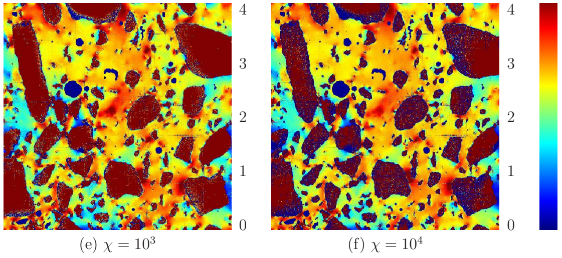
Figure 9: 2D sections of the normalized mean stress component \sigma_m/[E^{(m)}\langle\varepsilon_m\rangle] at varying contrasts \chi = E^{(a)}/E^{(m)} . The field maps are thresholded according to the color-scale as shown on the right. Hydrostatic strain loading is applied with \langle\varepsilon_m\rangle = \varepsilon_0 (colors on-line). The 3D image is of size 1.25 \times 1.25 \times 1.25 \text{ cm}^3 and of resolution 25 \text{ }\mu\text{m}/\text{voxel} .
