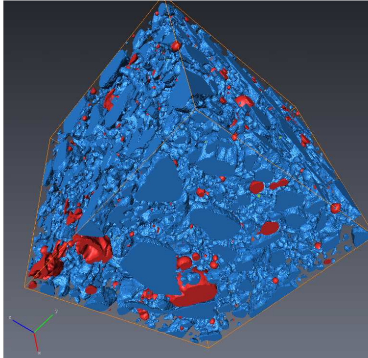
Figure 7: 3D microstructure: fine aggregates (blue) and voids (red). The matrix is transparent. The displayed volume is of size 1.25 \times 1.25 \times 1.25 \text{ cm}^3 , the image has been sub-sampled to a resolution of 31 \text{ }\mu\text{m}/\text{voxel} to do the mesh.
