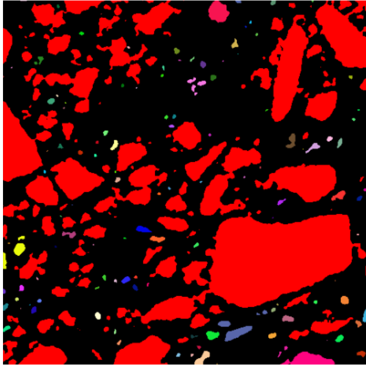
Figure 4: Image labeling of the segmented microstructure before disconnection of aggregates. Each color represents a connected component of the aggregates phase. Most aggregates are connected through a large percolating cluster (shown in red). In reality, aggregates are disconnected.
