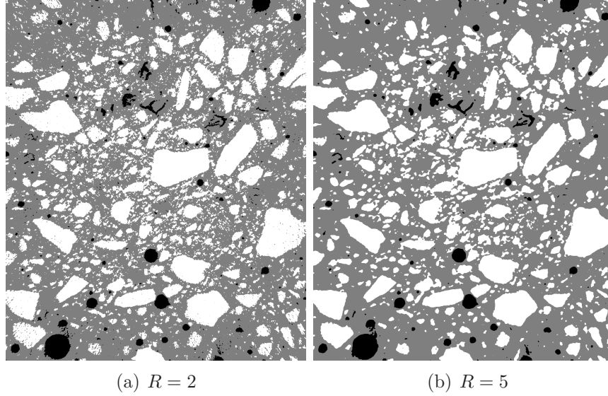
Figure 2: Examples of filtered and thresholded images at two filter sizes R = 2, 5 voxels: fine aggregates (white), voids (black) and matrix (gray). When the image noise is incompletely removed ( R = 2 , left), the aggregates specific surface area is overestimated.
