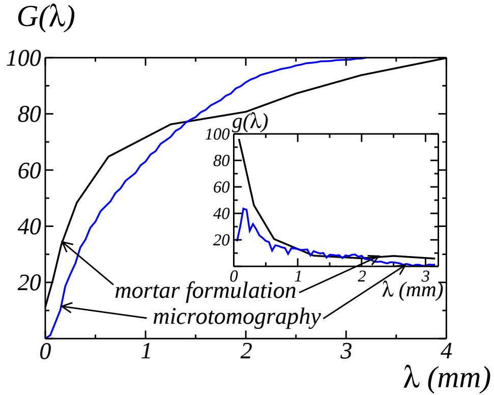
Figure 8: Cumulative fine aggregates size distribution G as a function of the diameter \lambda . The formulation of the mortar as well as the distribution deduced from the segmentation of the microtomography image are given. The fine aggregates size distribution g , which takes into account the volume fractions in the sample, is also given.
