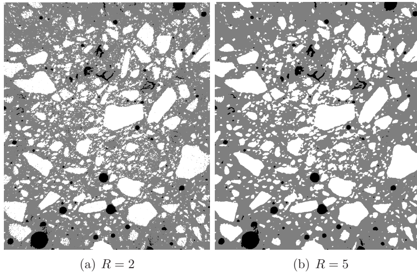
Figure 2: Examples of filtered and thresholded images at two filter sizes R = 2, 5 voxels: fine aggregates (white), voids (black) and matrix (gray). When the image noise is incompletely removed ( R = 2 , left), the aggregates specific surface area is overestimated.
