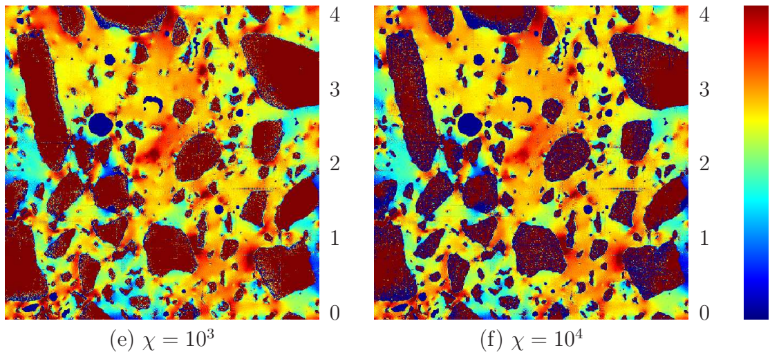
Figure 9: 2D sections of the normalized mean stress component \sigma_m/[E^{(m)}\langle\varepsilon_m\rangle] at varying contrasts \chi = E^{(a)}/E^{(m)} . The field maps are thresholded according to the color-scale as shown on the right. Hydrostatic strain loading is applied with \langle\varepsilon_m\rangle = \varepsilon_0 (colors on-line). The 3D image is of size 1.25 \times 1.25 \times 1.25 \text{ cm}^3 and of resolution 25 \text{ }\mu\text{m}/\text{voxel} .
