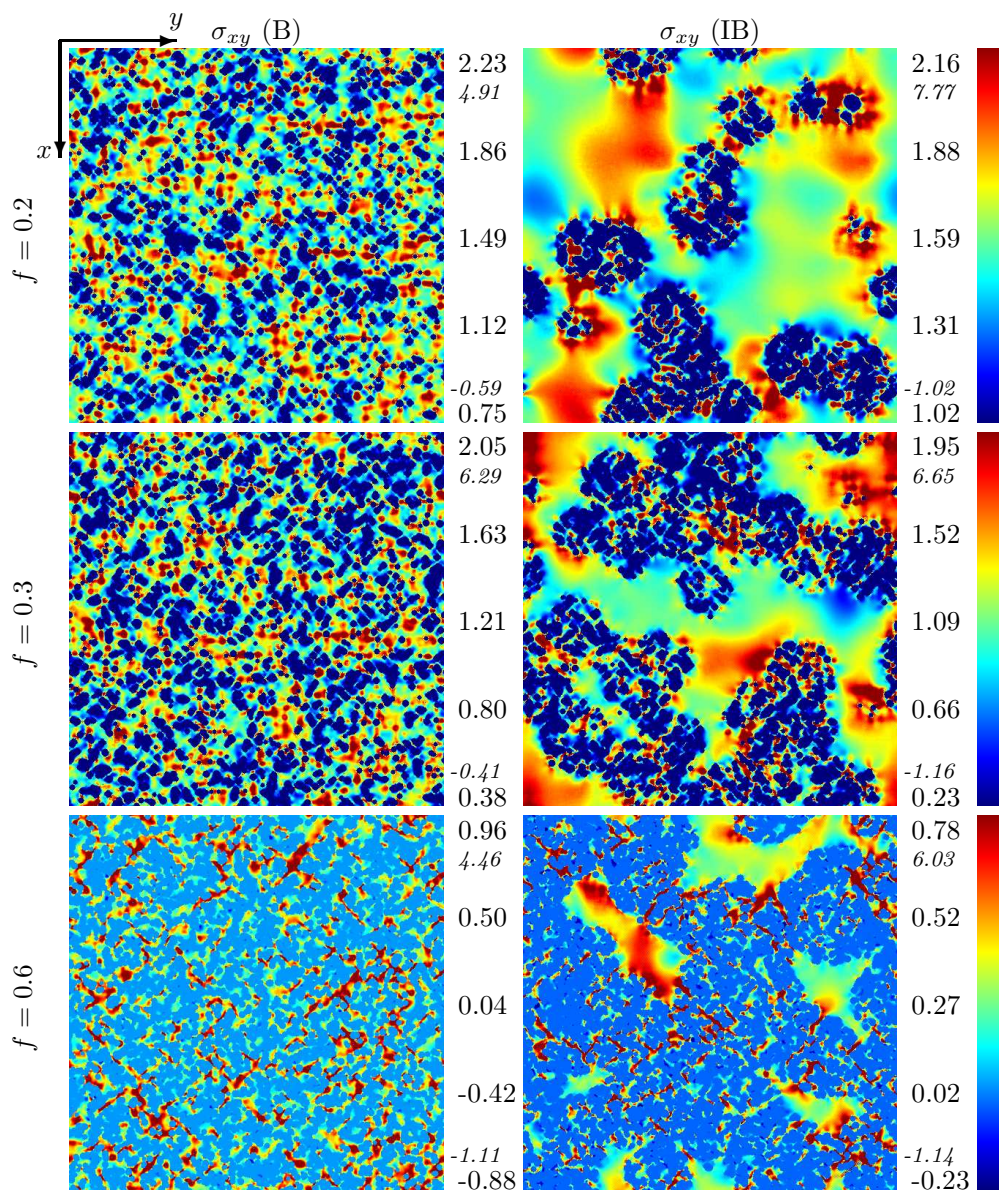
FIG. 10.11. Continuation of Fig. 10.10: component \sigma_{xy} , with applied strain shear loading \langle \varepsilon_{xy} \rangle = 1 .
