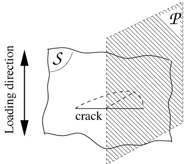
Fig. 6. Relative position of the specimen surface S and the plane of observation P.
