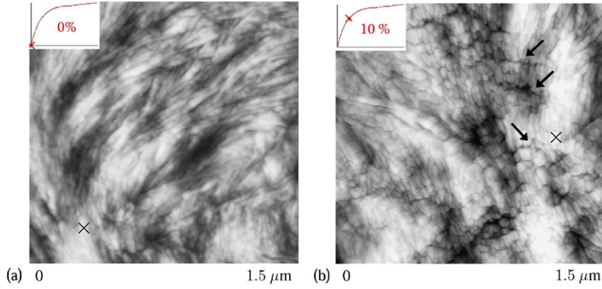
Fig. 1. (a) AFM height image of undeformed PB ( \Delta l/l_0 = 0\% ); (b) AFM height image of deformed PB \Delta l/l_0 = 10\% ( Z_{\text{range}} = 120 \text{ nm} ) [9].
