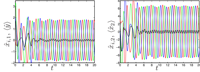
(a) Outputs \hat{y}_i (= \hat{x}_{i,1}) , i = 1, 2, 3 (red, green, blue, respectively), and \langle \hat{y} \rangle (black). (b) Components \hat{x}_{i,2} , i = 1, 2, 3 (red, green, blue, respectively), and \langle \hat{x}_2 \rangle (black).
